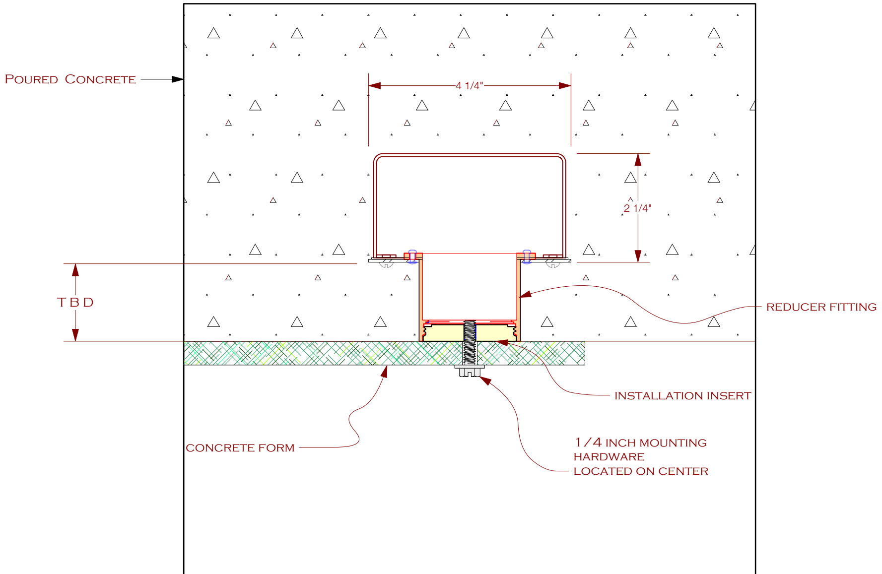
INSTALLATION DETAIL
